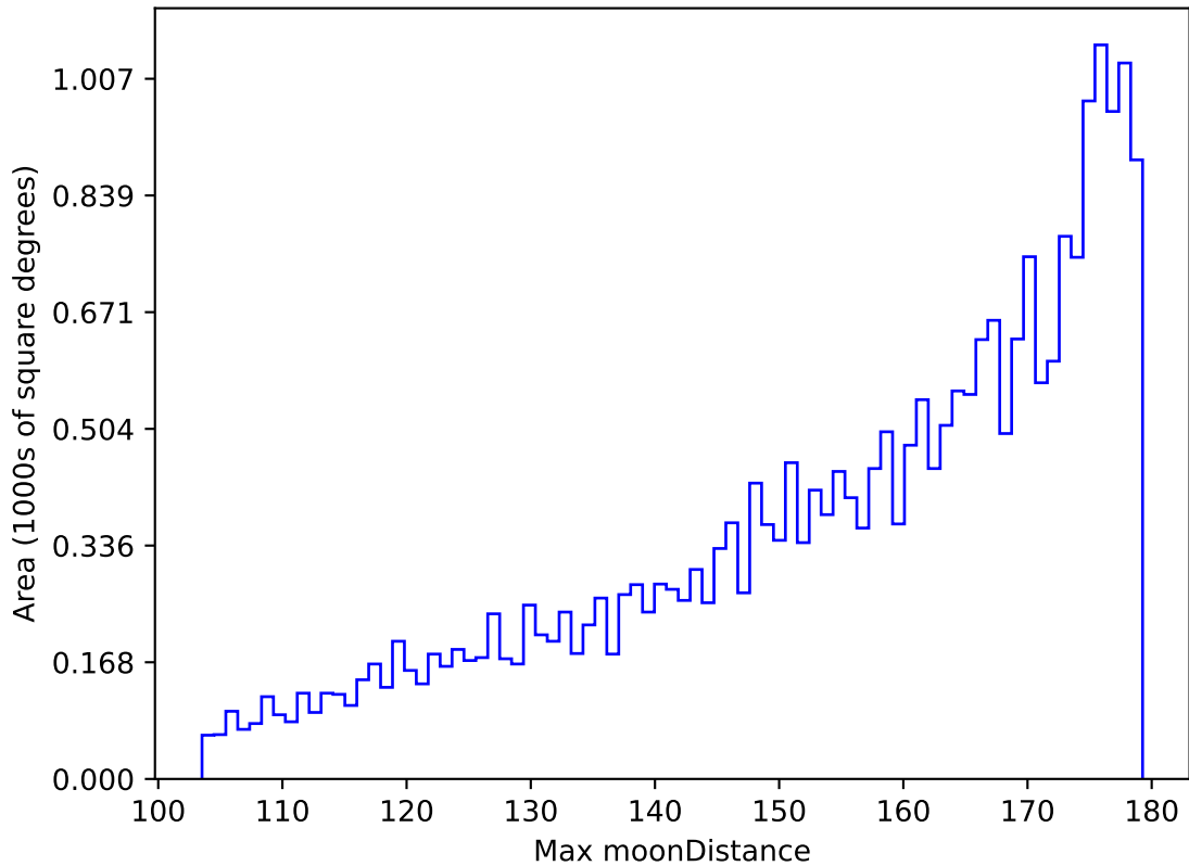
too_elab_r8_d3_giz_v3.4_10yrs All sky i band: Max moonDistance
