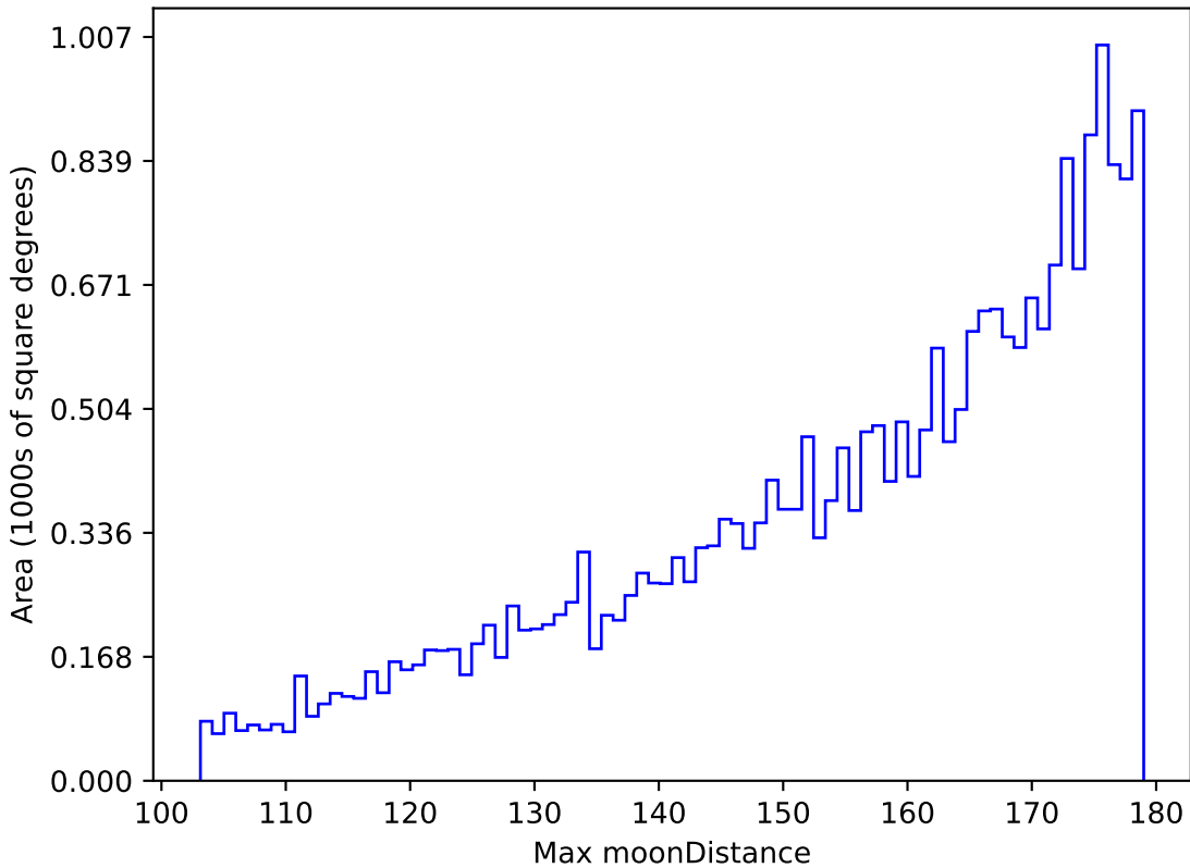
too_elab_r8_d3_giz_v3.4_10yrs All sky g band: Max moonDistance
