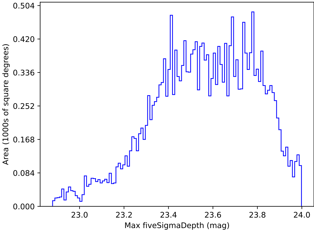
too_elab_r8_d3_giz_v3.4_10yrs Yr 1 u band: Max fiveSigmaDepth
