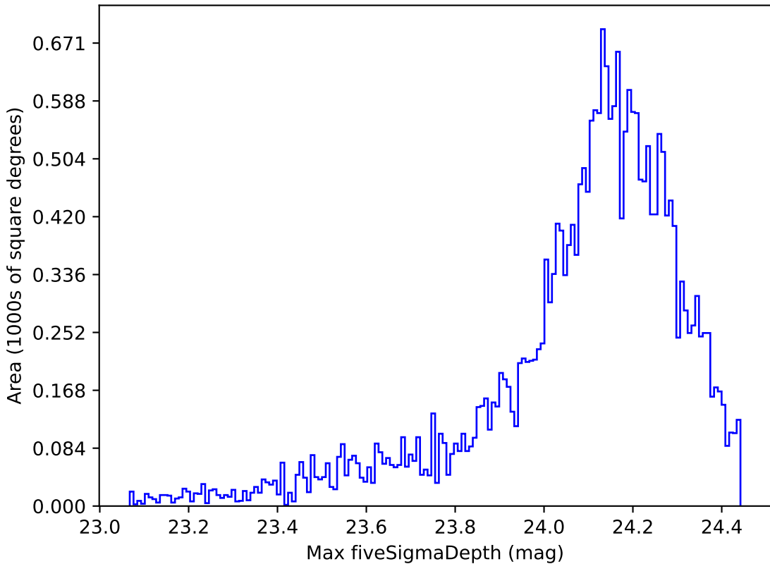
too_elab_r8_d3_giz_v3.4_10yrs Yr 1 i band: Max fiveSigmaDepth
