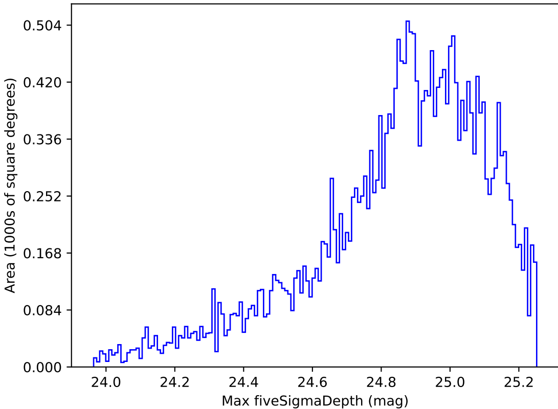
too_elab_r8_d3_giz_v3.4_10yrs Yr 1 g band: Max fiveSigmaDepth
