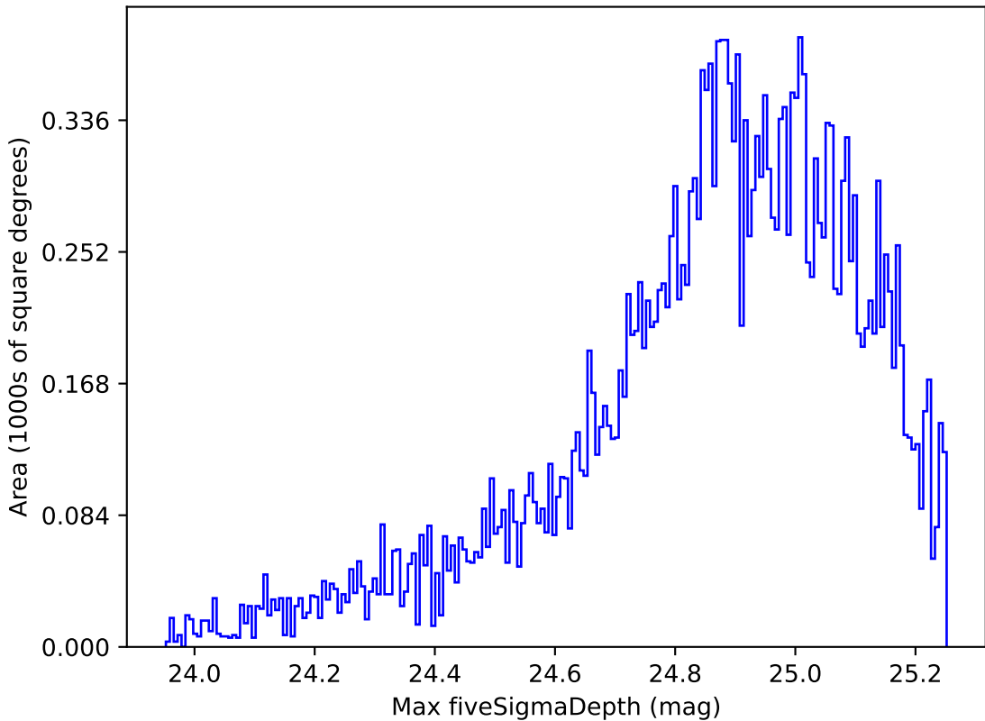
too_elab_r8_d3_giz_v3.4_10yrs Yr 1 all bands: Max fiveSigmaDepth
