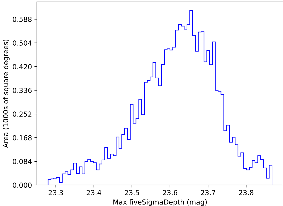
too_elab_r8_d3_giz_v3.4_10yrs WFD z band: Max fiveSigmaDepth
