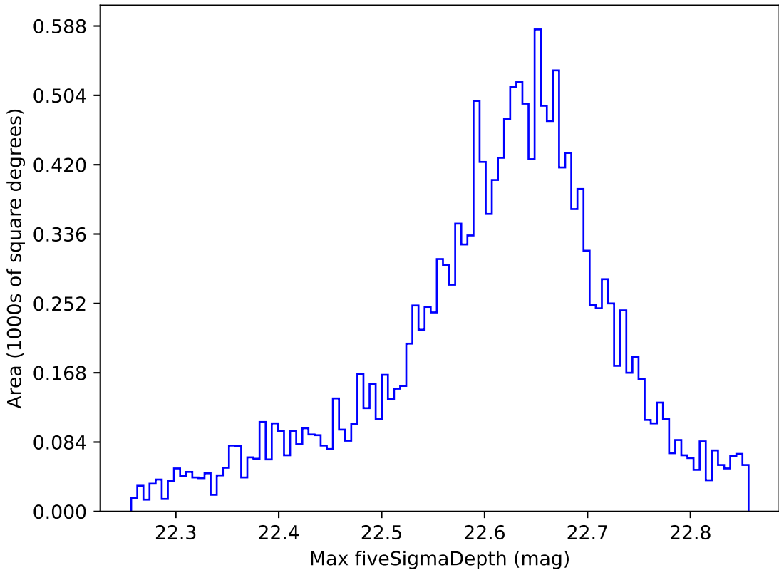
too_elab_r8_d3_giz_v3.4_10yrs WFD y band: Max fiveSigmaDepth
