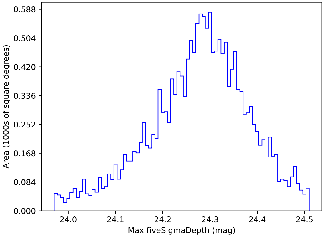
too_elab_r8_d3_giz_v3.4_10yrs WFD i band: Max fiveSigmaDepth
