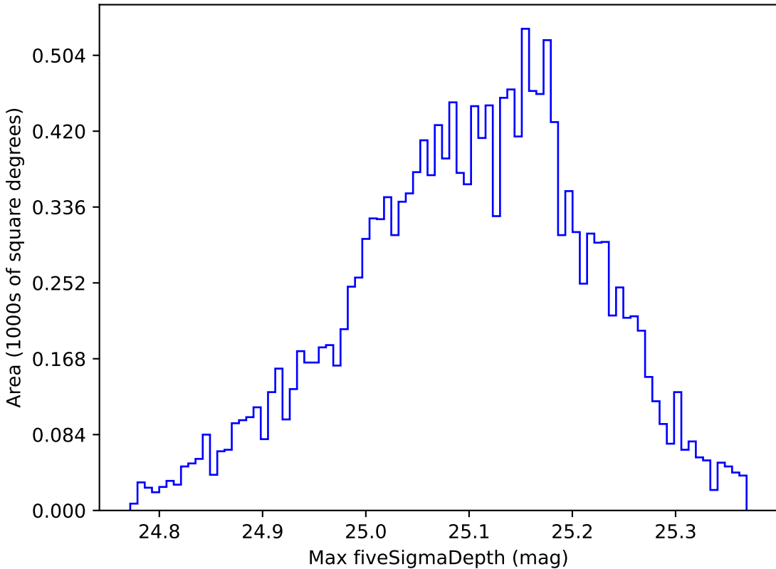
too_elab_r8_d3_giz_v3.4_10yrs WFD g band: Max fiveSigmaDepth
