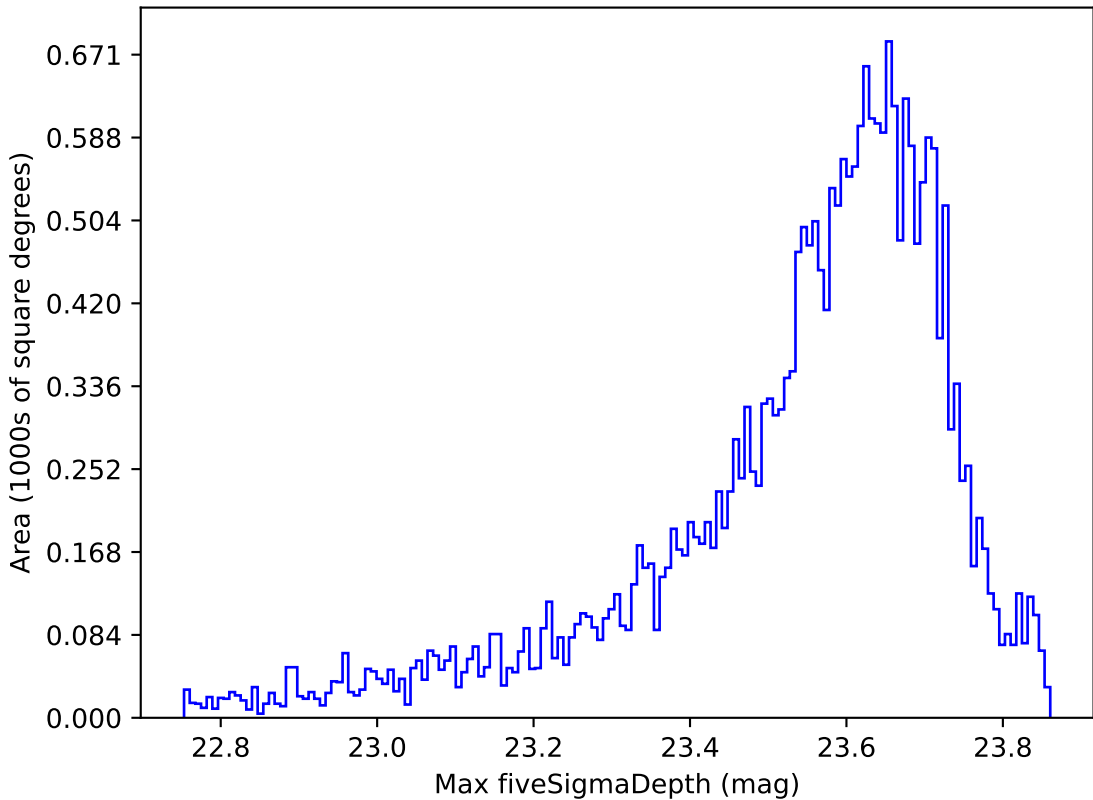
too_elab_r8_d3_giz_v3.4_10yrs All sky z band: Max fiveSigmaDepth
