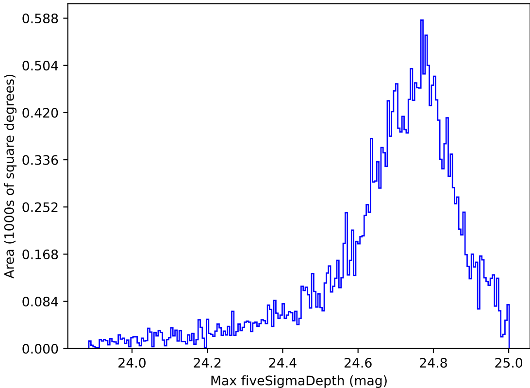
too_elab_r8_d3_giz_v3.4_10yrs All sky r band: Max fiveSigmaDepth
