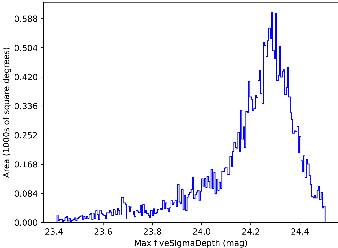
too_elab_r8_d3_giz_v3.4_10yrs All sky i band: Max fiveSigmaDepth
