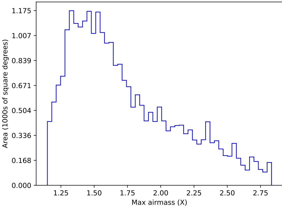
too_elab_r8_d3_giz_v3.4_10yrs Yr 1 z band: Max airmass
