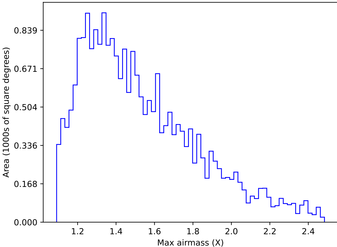
too_elab_r8_d3_giz_v3.4_10yrs Yr 1 u band: Max airmass
