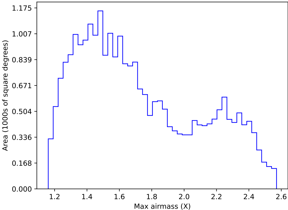
too_elab_r8_d3_giz_v3.4_10yrs Yr 1 r band: Max airmass
