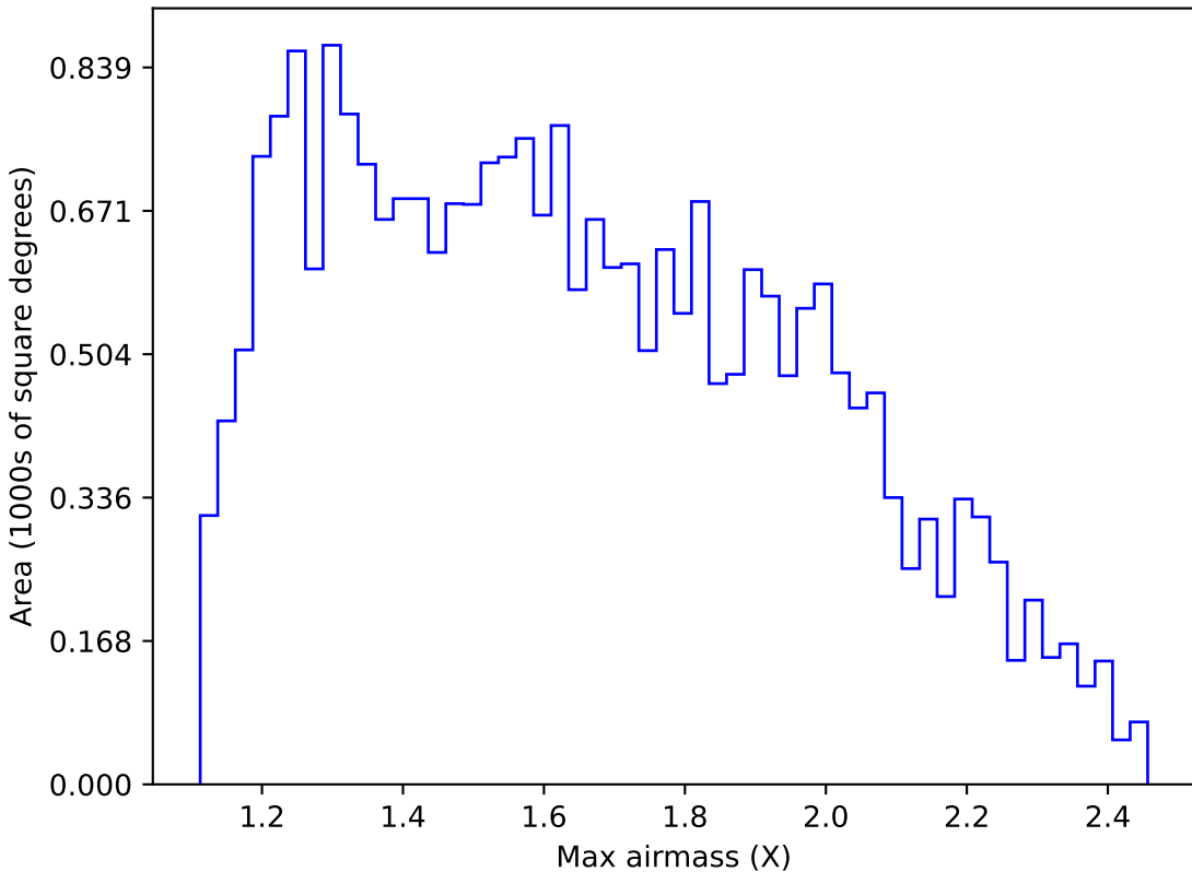
too_elab_r8_d3_giz_v3.4_10yrs Yr 1 g band: Max airmass
