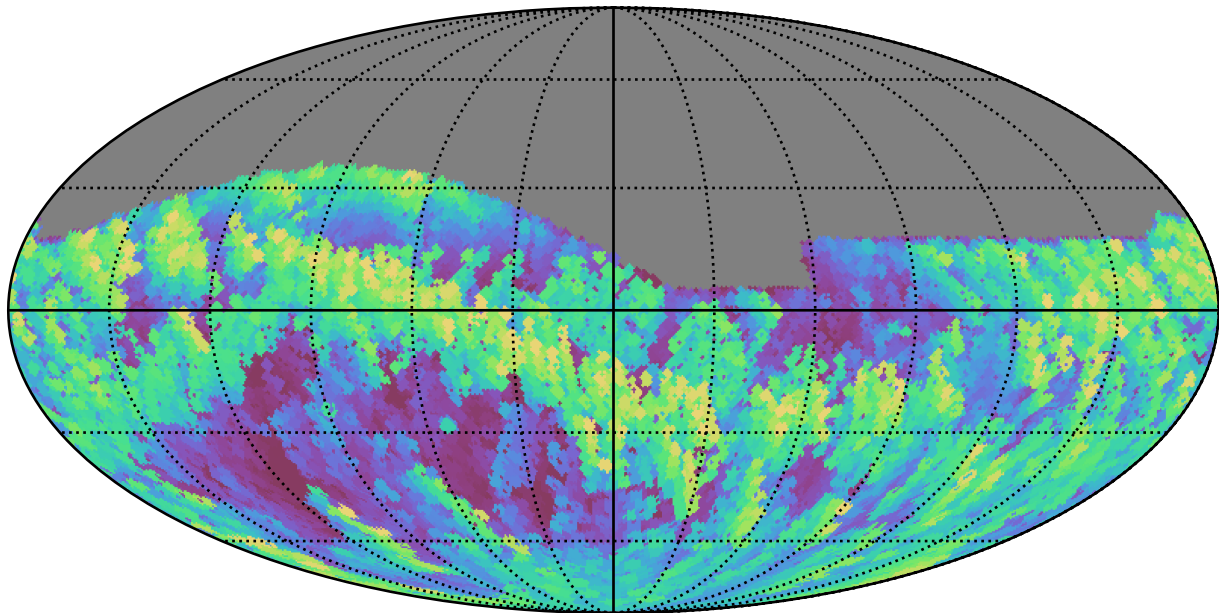
too_elab_r8_d3_giz_v3.4_10yrs Yr 1 all bands: Max airmass
