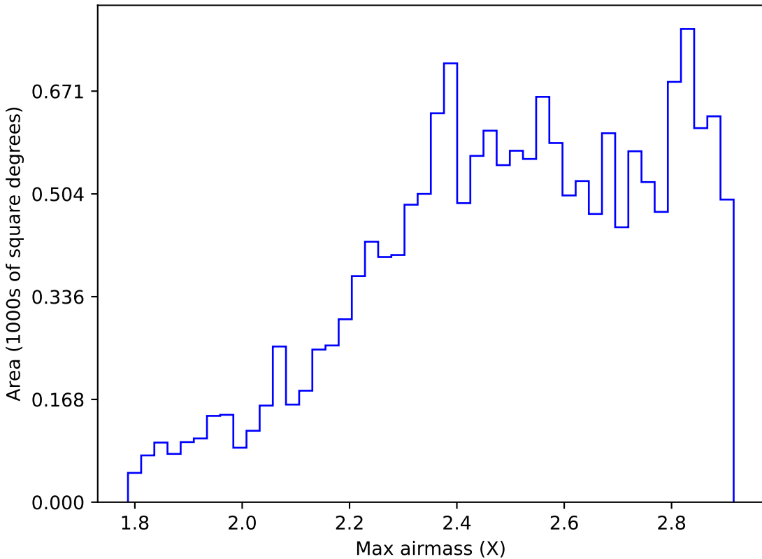
too_elab_r8_d3_giz_v3.4_10yrs WFD z band: Max airmass
