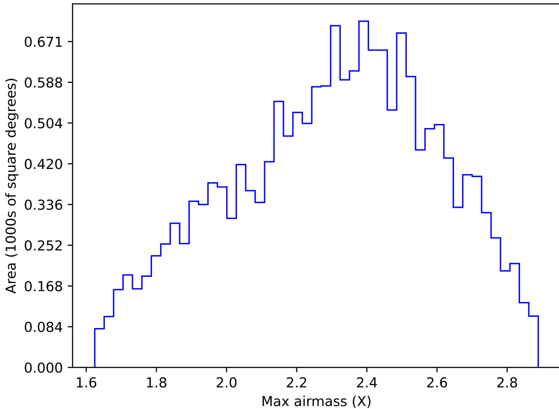
too_elab_r8_d3_giz_v3.4_10yrs WFD y band: Max airmass
