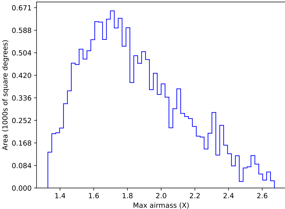
too_elab_r8_d3_giz_v3.4_10yrs WFD u band: Max airmass
