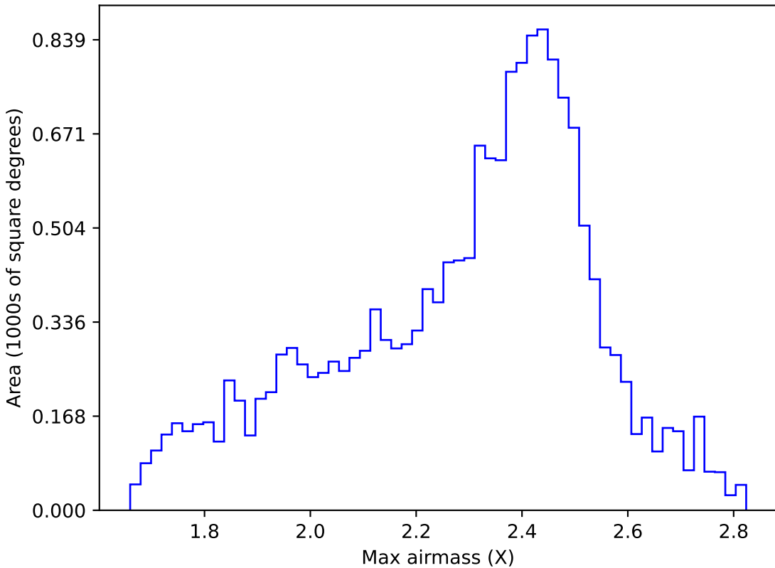
too_elab_r8_d3_giz_v3.4_10yrs WFD r band: Max airmass
