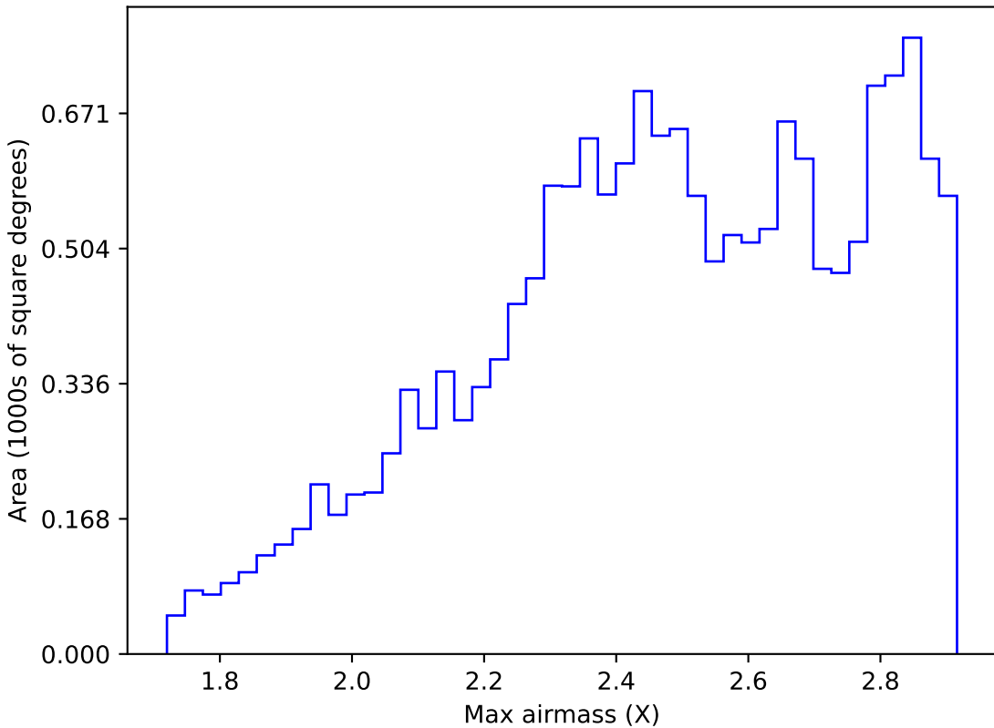
too_elab_r8_d3_giz_v3.4_10yrs WFD i band: Max airmass
