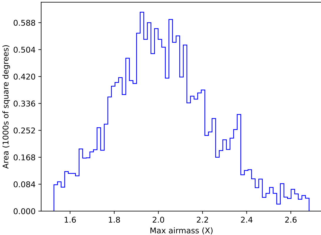
too_elab_r8_d3_giz_v3.4_10yrs WFD g band: Max airmass
