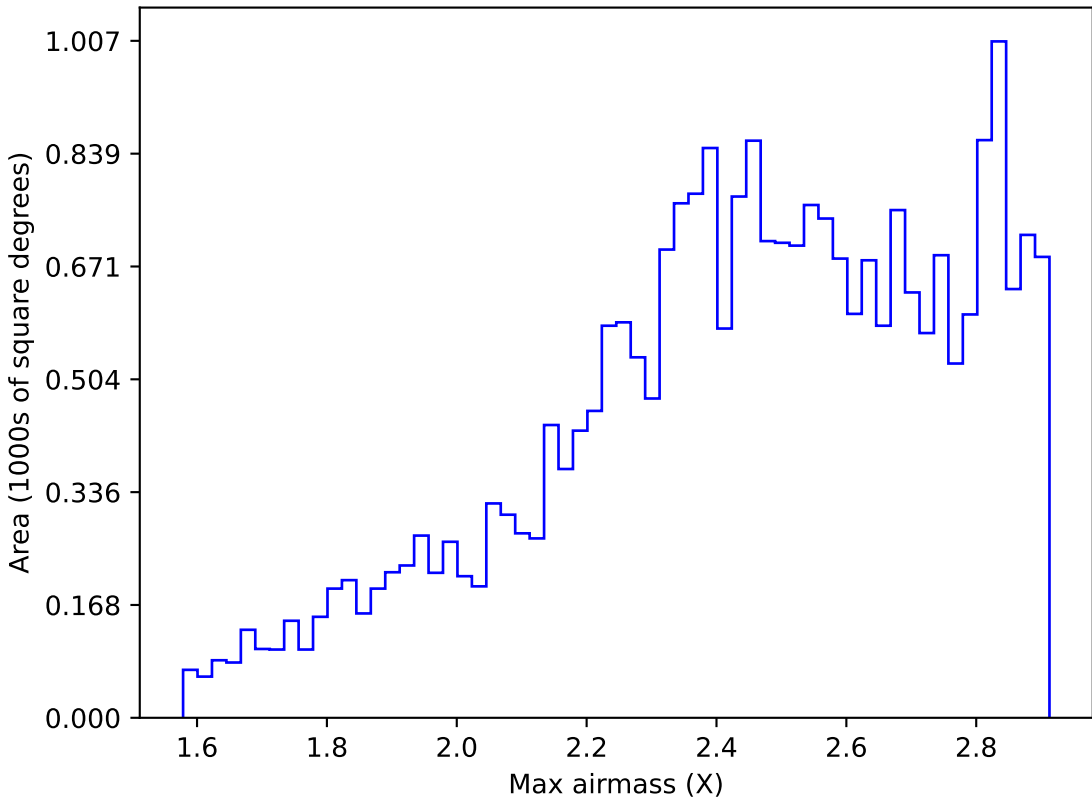
too_elab_r8_d3_giz_v3.4_10yrs All sky z band: Max airmass
