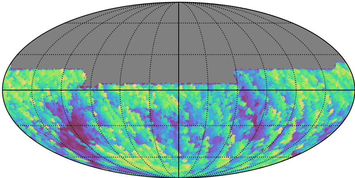
too_elab_r8_d3_giz_v3.4_10yrs All sky y band: Max airmass
