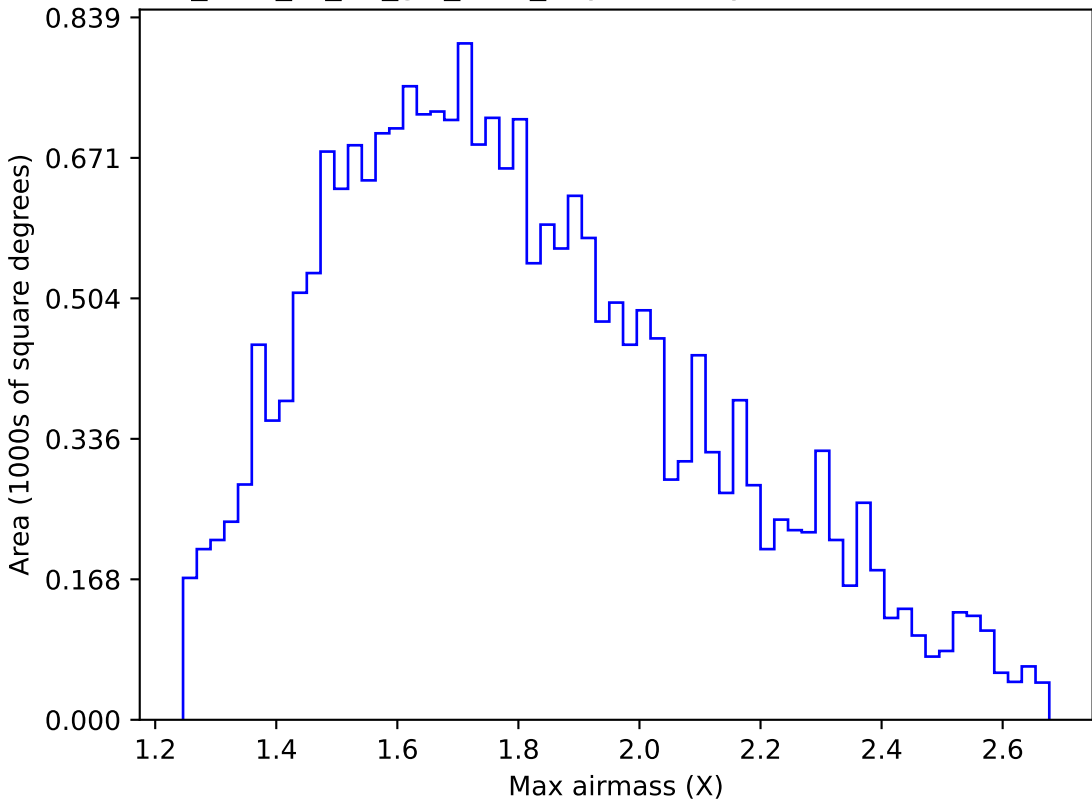
too_elab_r8_d3_giz_v3.4_10yrs All sky u band: Max airmass
