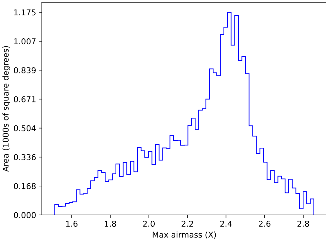
too_elab_r8_d3_giz_v3.4_10yrs All sky r band: Max airmass
