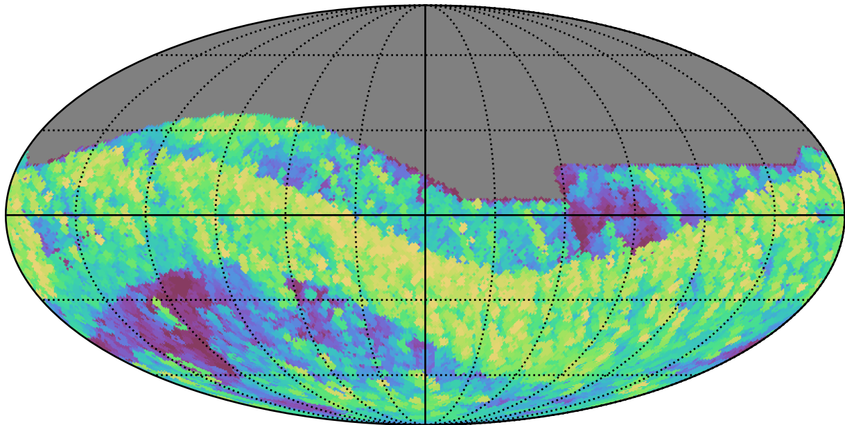
too_elab_r8_d3_giz_v3.4_10yrs All sky i band: Max airmass
