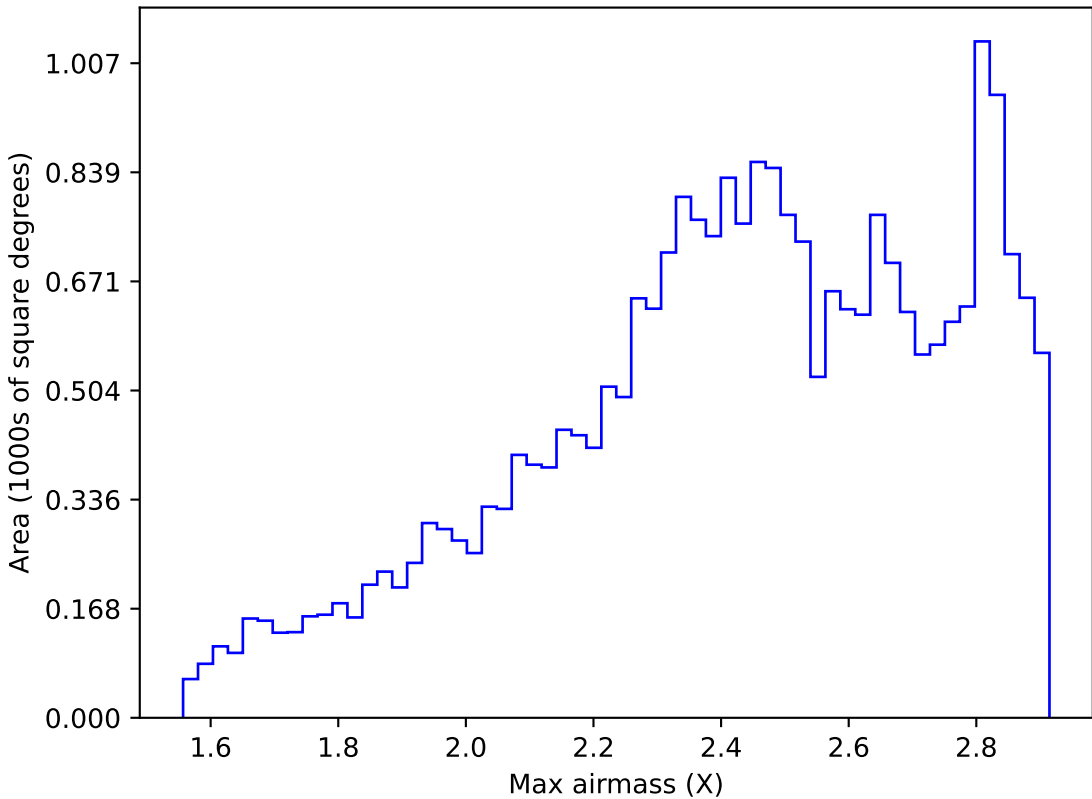
too_elab_r8_d3_giz_v3.4_10yrs All sky i band: Max airmass
