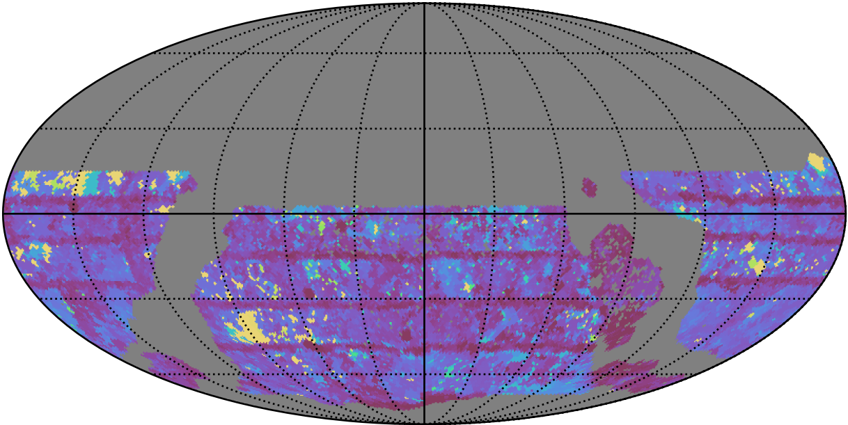
too_elab_r8_d3_giz_v3.4_10yrs WFD z band: Max Inter-Night Gap
