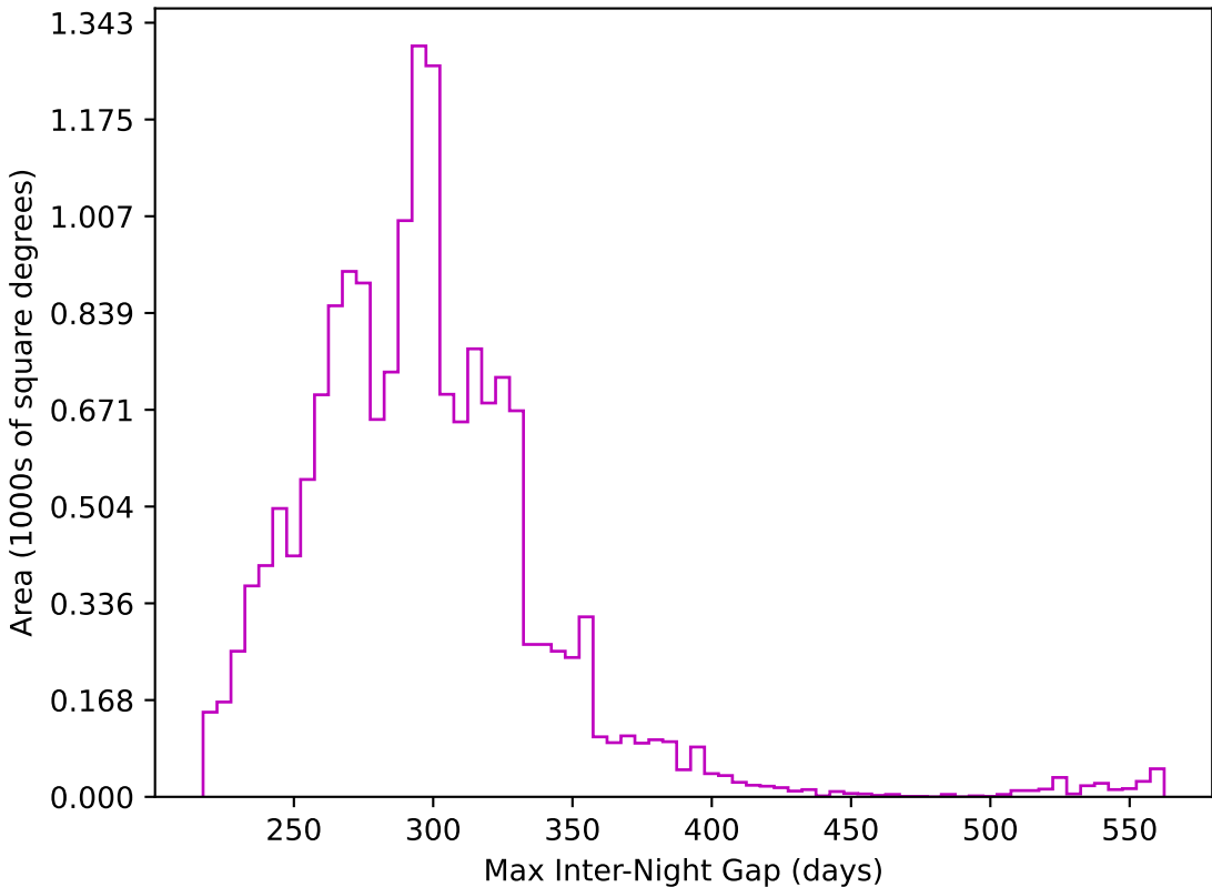
too_elab_r8_d3_giz_v3.4_10yrs WFD z band: Max Inter-Night Gap
