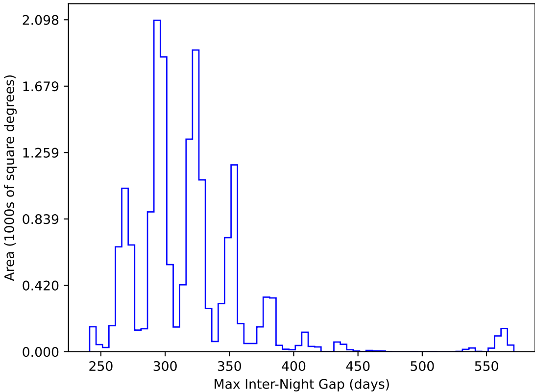
too_elab_r8_d3_giz_v3.4_10yrs WFD y band: Max Inter-Night Gap
