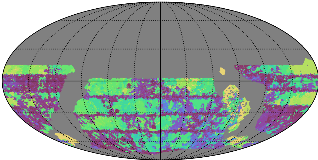
too_elab_r8_d3_giz_v3.4_10yrs WFD u band: Max Inter-Night Gap
