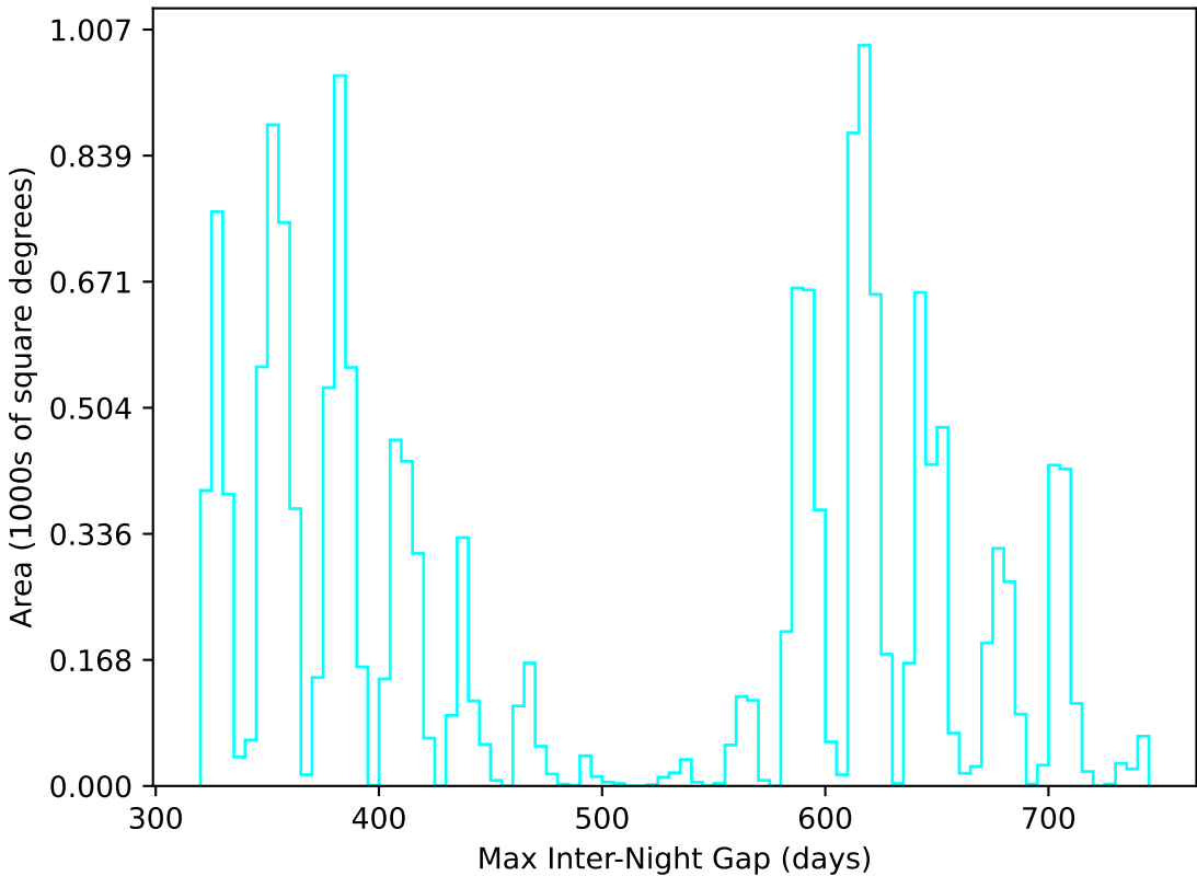
too_elab_r8_d3_giz_v3.4_10yrs WFD u band: Max Inter-Night Gap
