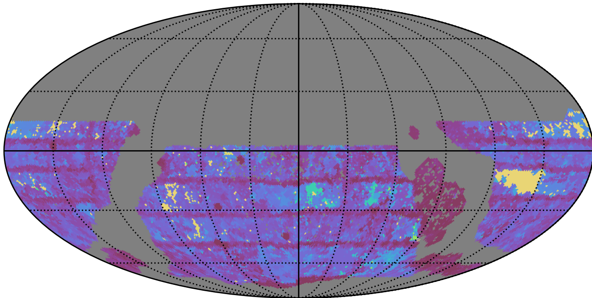
too_elab_r8_d3_giz_v3.4_10yrs WFD r band: Max Inter-Night Gap
