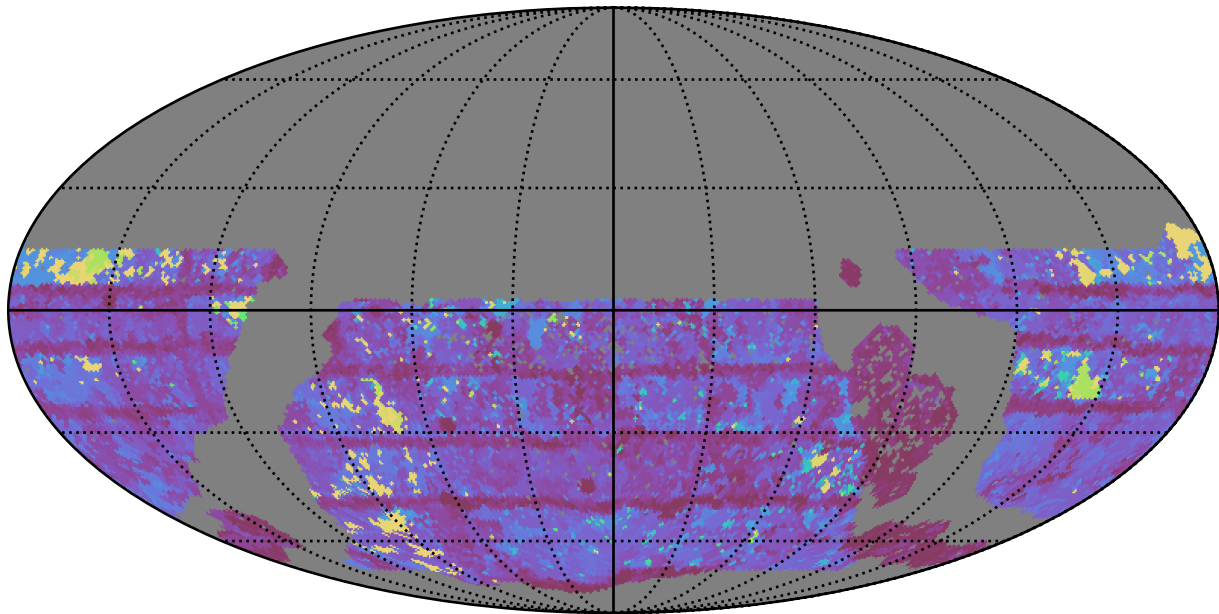
too_elab_r8_d3_giz_v3.4_10yrs WFD i band: Max Inter-Night Gap
