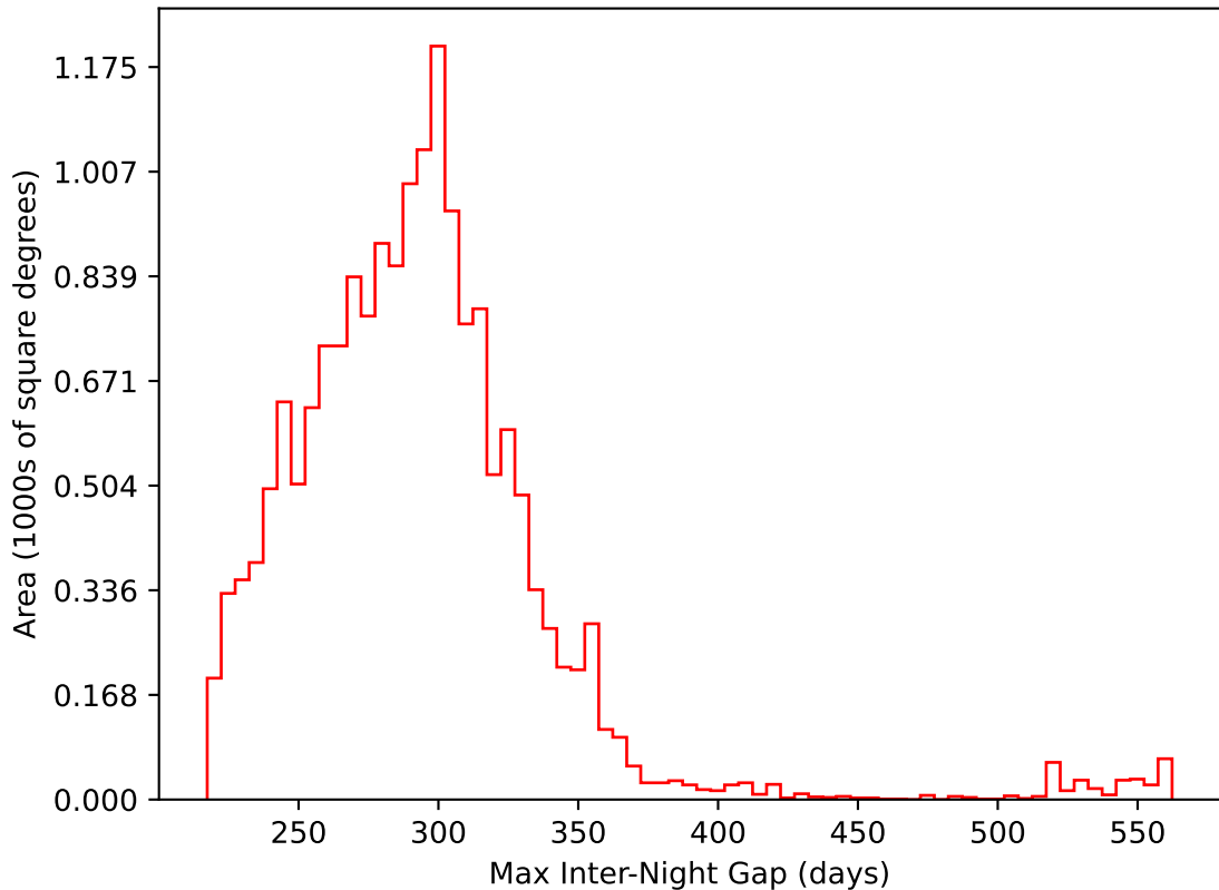
too_elab_r8_d3_giz_v3.4_10yrs WFD i band: Max Inter-Night Gap
