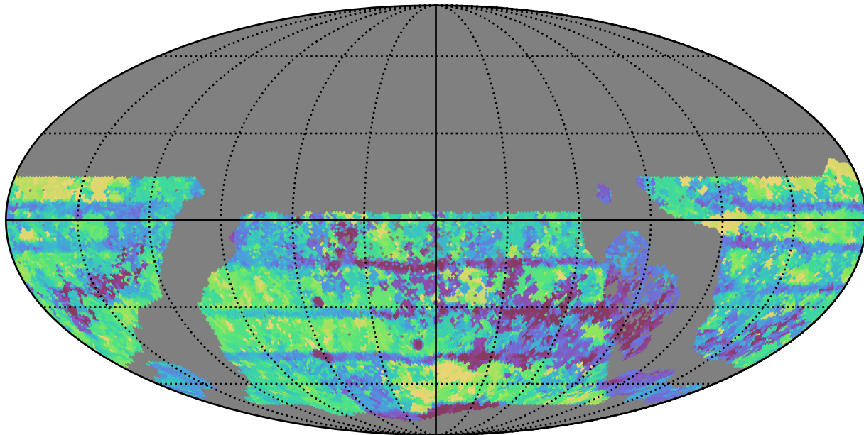
too_elab_r8_d3_giz_v3.4_10yrs WFD all bands: Max Inter-Night Gap
