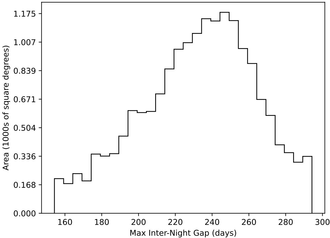
too_elab_r8_d3_giz_v3.4_10yrs WFD all bands: Max Inter-Night Gap
