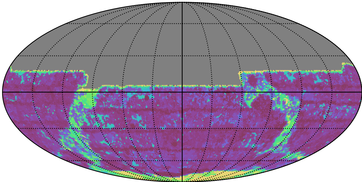
too_elab_r8_d3_giz_v3.4_10yrs All sky y band: Max Inter-Night Gap
