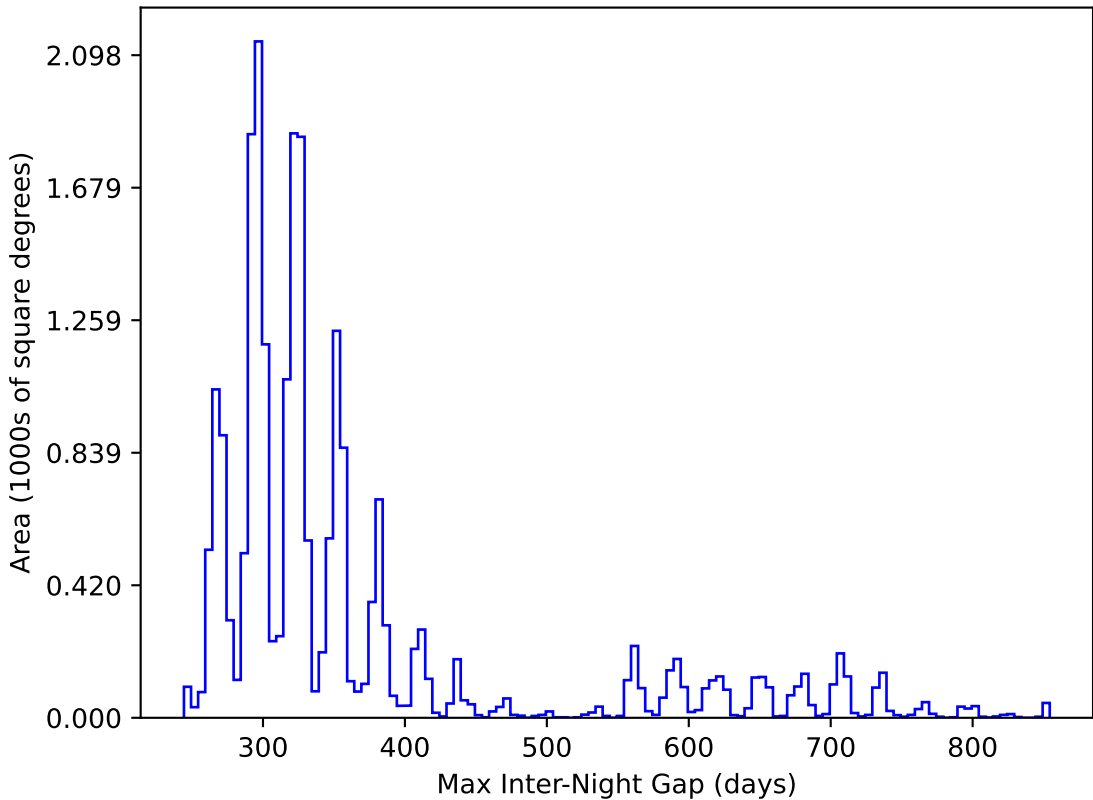
too_elab_r8_d3_giz_v3.4_10yrs All sky y band: Max Inter-Night Gap
