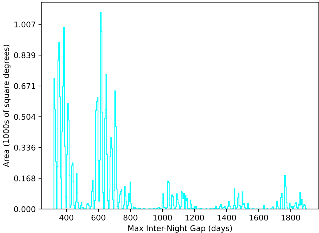
too_elab_r8_d3_giz_v3.4_10yrs All sky u band: Max Inter-Night Gap
