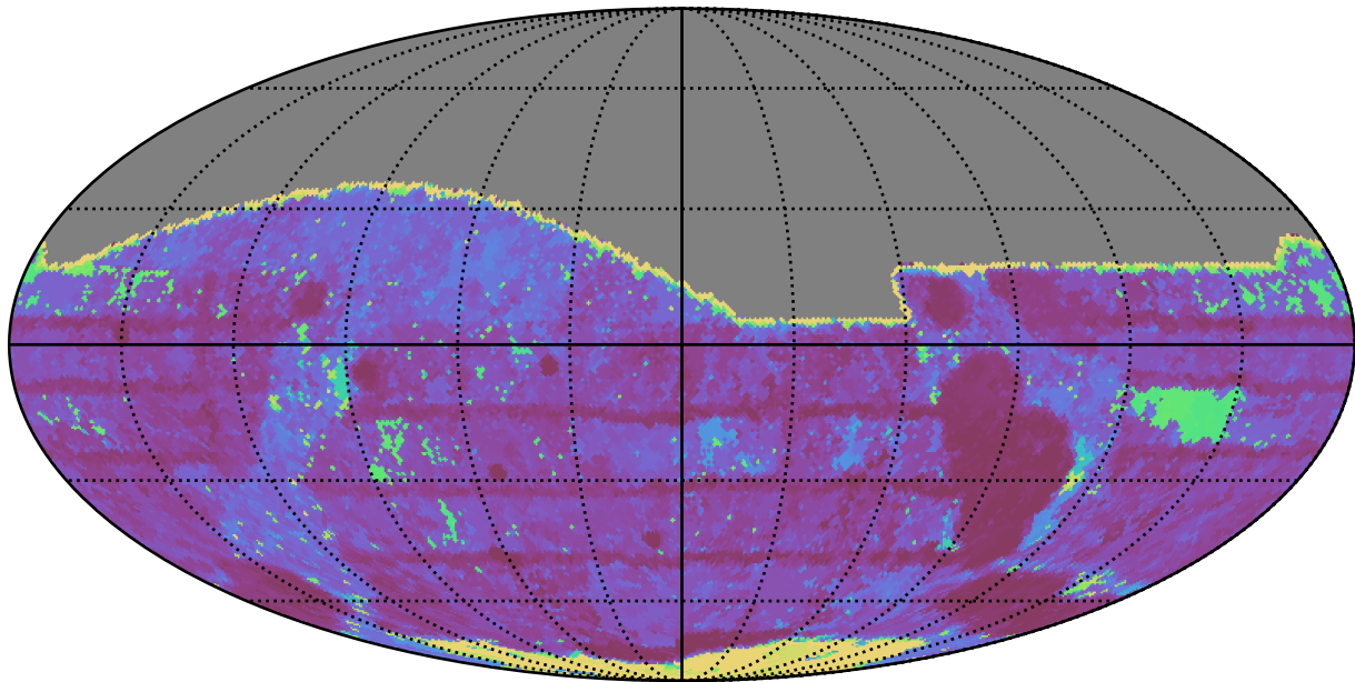
too_elab_r8_d3_giz_v3.4_10yrs All sky r band: Max Inter-Night Gap
