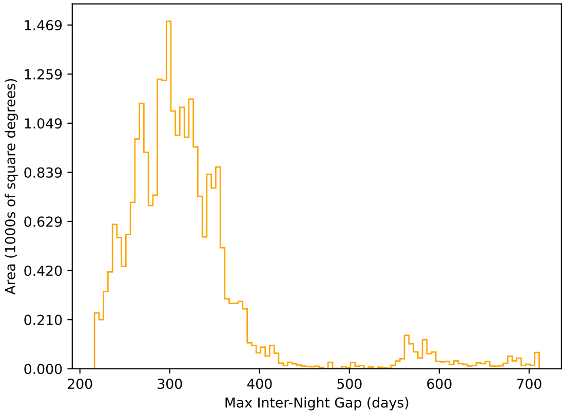
too_elab_r8_d3_giz_v3.4_10yrs All sky r band: Max Inter-Night Gap
