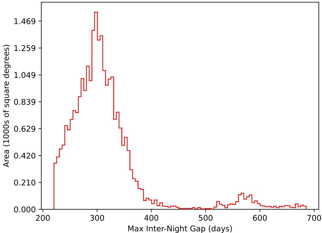
too_elab_r8_d3_giz_v3.4_10yrs All sky i band: Max Inter-Night Gap
