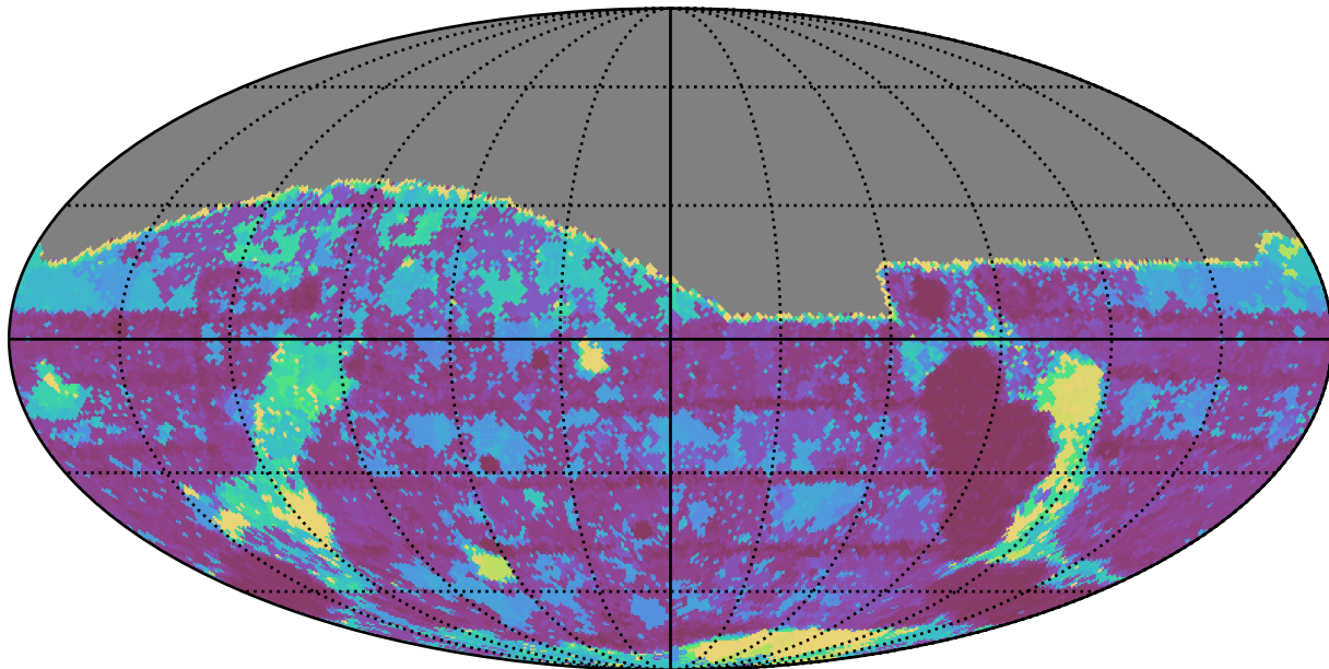
too_elab_r8_d3_giz_v3.4_10yrs All sky g band: Max Inter-Night Gap
