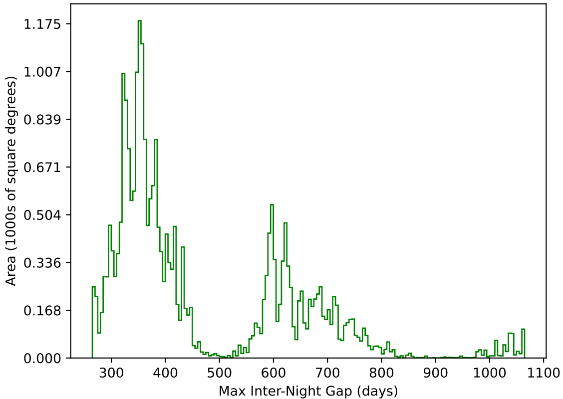
too_elab_r8_d3_giz_v3.4_10yrs All sky g band: Max Inter-Night Gap
