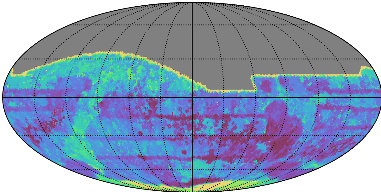
too_elab_r8_d3_giz_v3.4_10yrs All sky all bands: Max Inter-Night Gap
