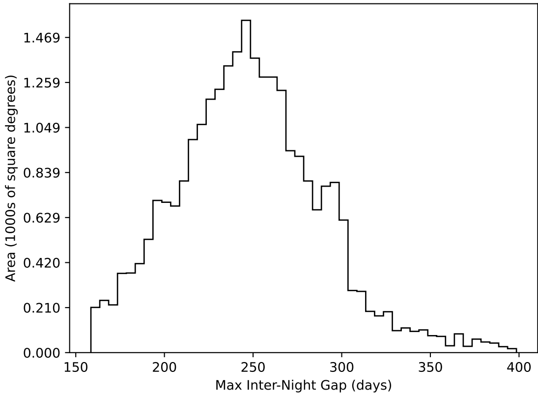
too_elab_r8_d3_giz_v3.4_10yrs All sky all bands: Max Inter-Night Gap
